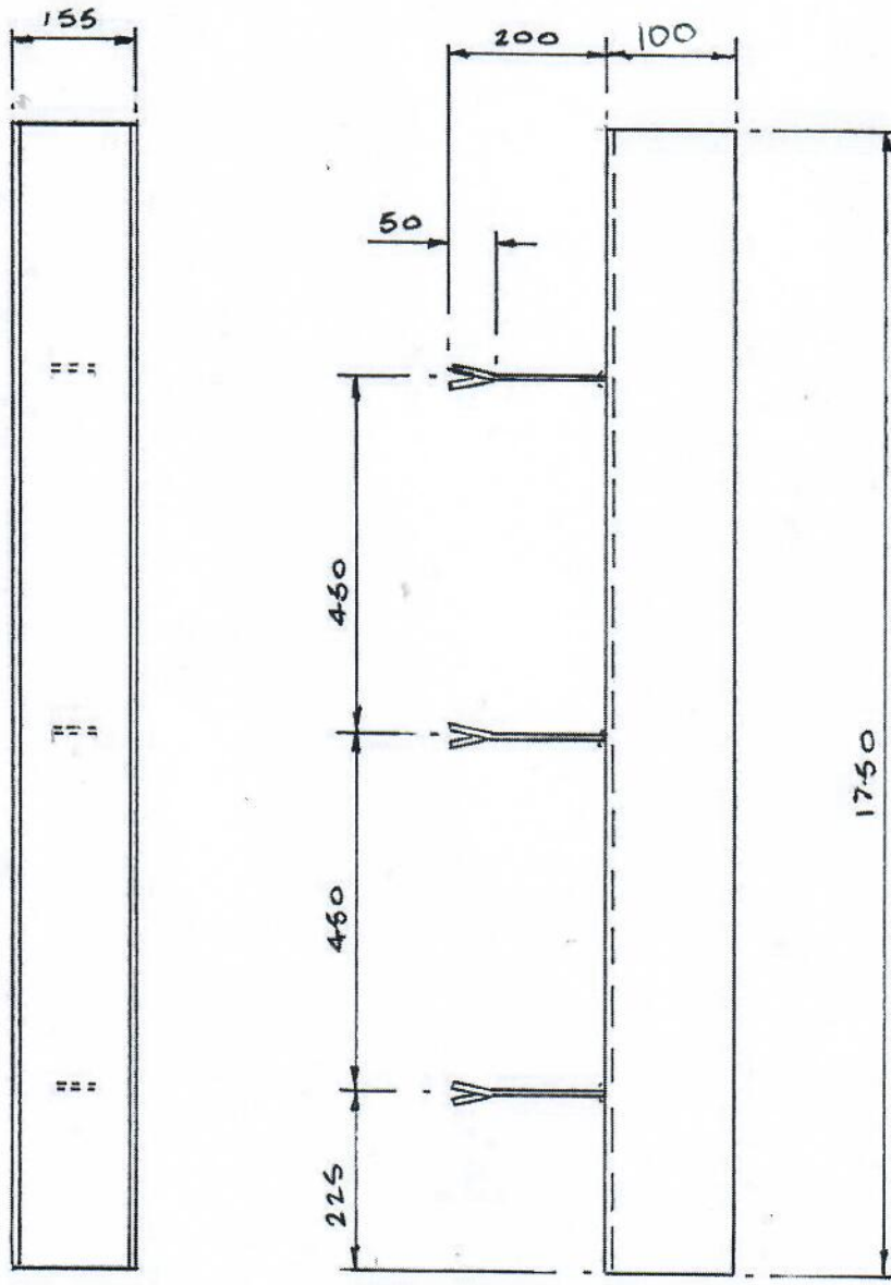
FRONT ELEVATION 1:10
